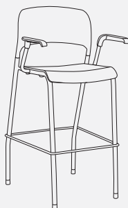
Rover café stool with arms W 695 x D 625 x H 1210
